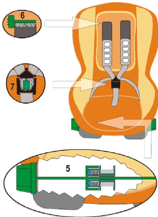
Figure 6: Belt Tension System
