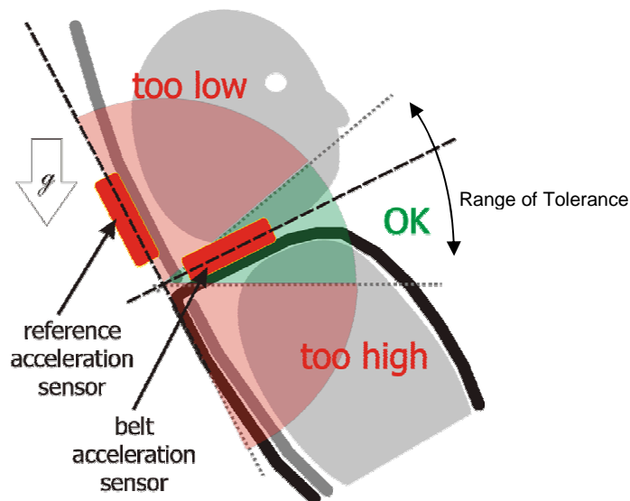
Figure 7: Principle of Shoulder sensor
