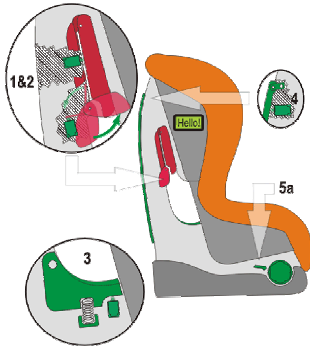
Figure 5: Belt Detection and Display
