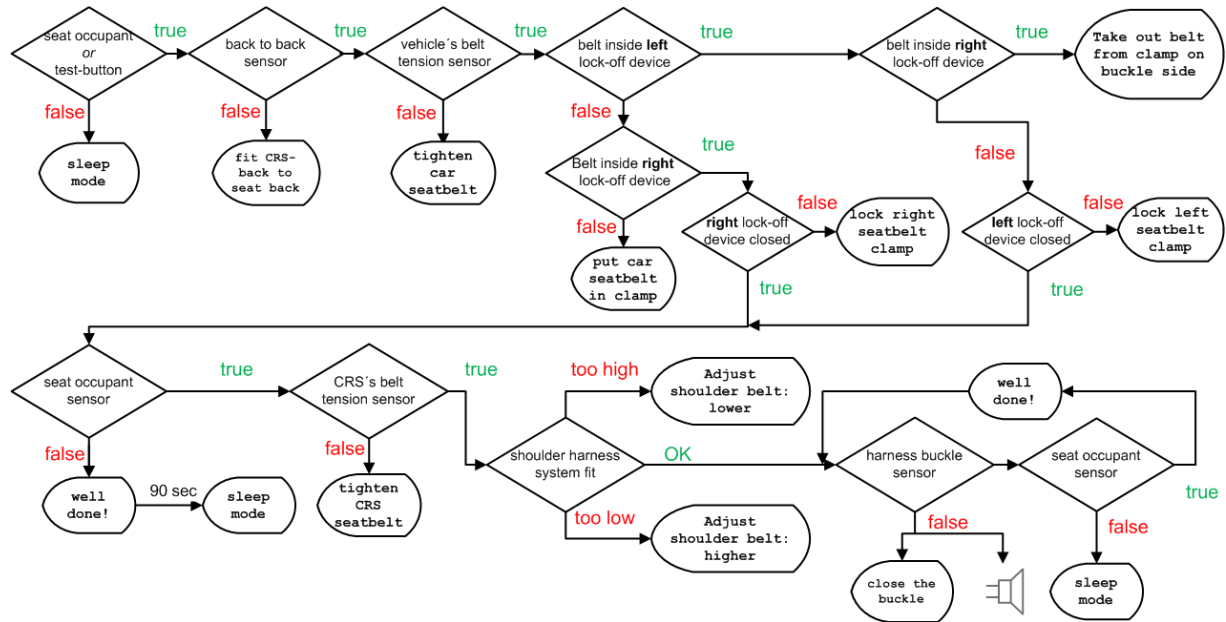
Figure 9: Schematic Diagram of Misuse check
